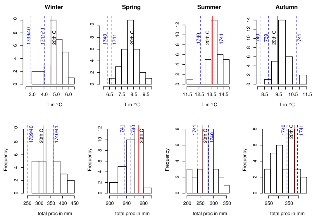
Fig. 3. Seasonal climate diagrams for Ireland (averaged over land only grid cells 51^{\circ} N– 56^{\circ} N, 11^{\circ} W– 5^{\circ} W). The histograms show temperatures (top panels) and seasonal precipitation (1710–1739). Solid red lines mark 1961–1990 averages; dashed blue lines denote values for seasons during the famine, years marked adjacent. Data from Luterbacher et al. (2000, 2004, 2007), Xoplaki et al. (2005) and Pauling et al. (2006).
