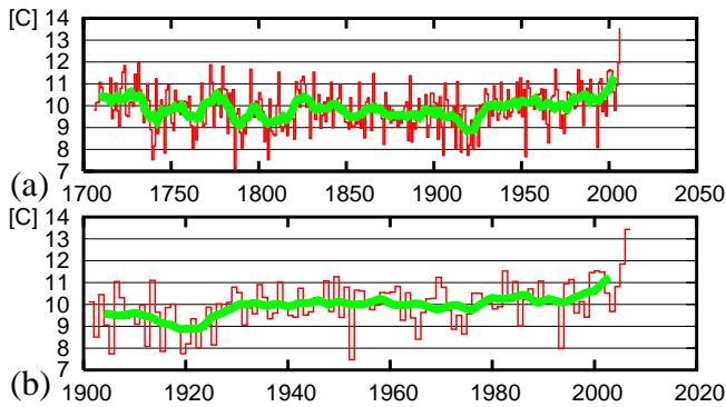
Fig. 1. Autumn 2-meter temperatures at De Bilt, the Netherlands with a 10-yr running mean (green) 1706–2006 (a, van Engelen and Nellesstijn, 1996), 1901–2006 corrected for changes in the thermometer hut, location and city effects (b, Verbeek, 2003).
